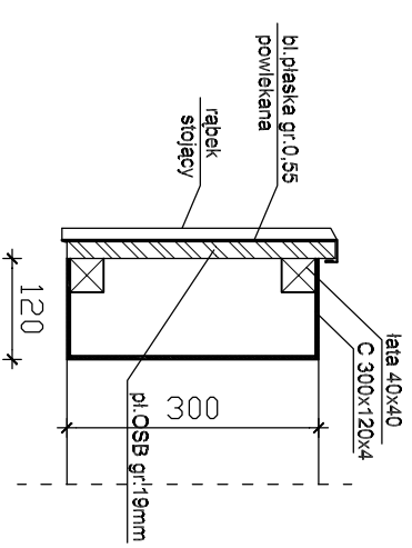
DETAIL "A" 1:10
